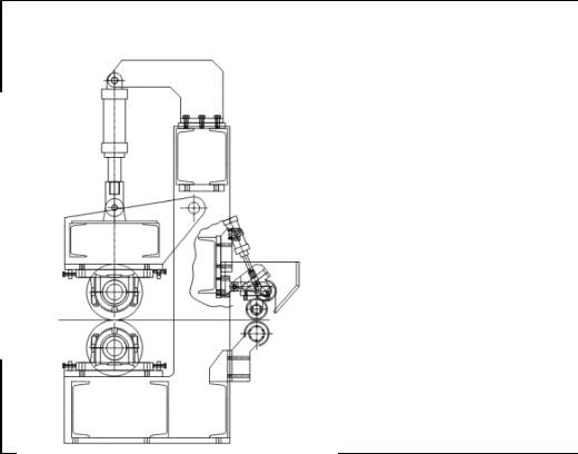
Feed Roll
