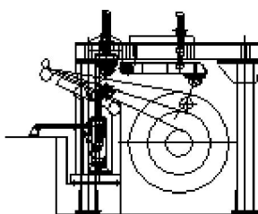
Entry Section
